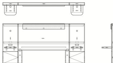
► PC221 KING HEADBOARD 123"W X 19"D X 60"H
